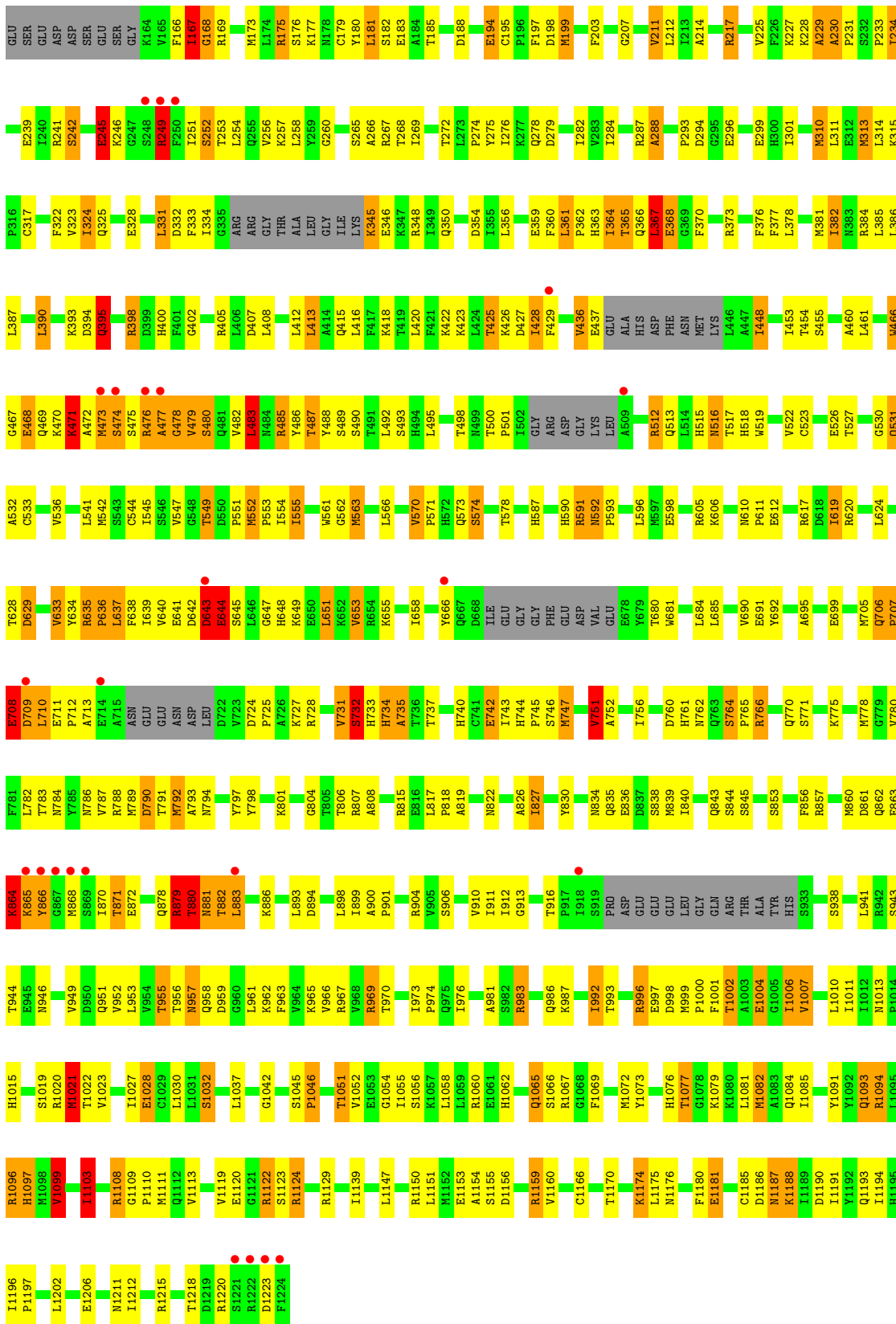
• Molecule 3: DNA-directed RNA polymerase II subunit RPB3
