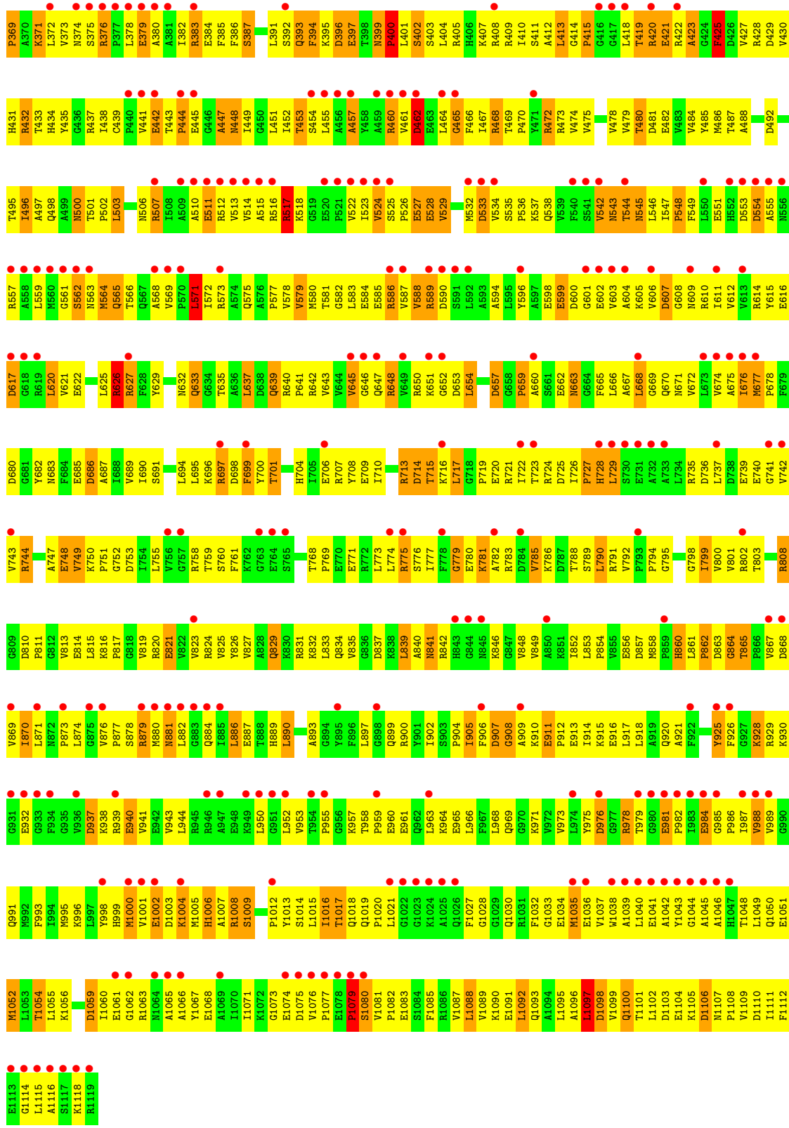
● Molecule 3: DNA-directed RNA polymerase beta' chain
