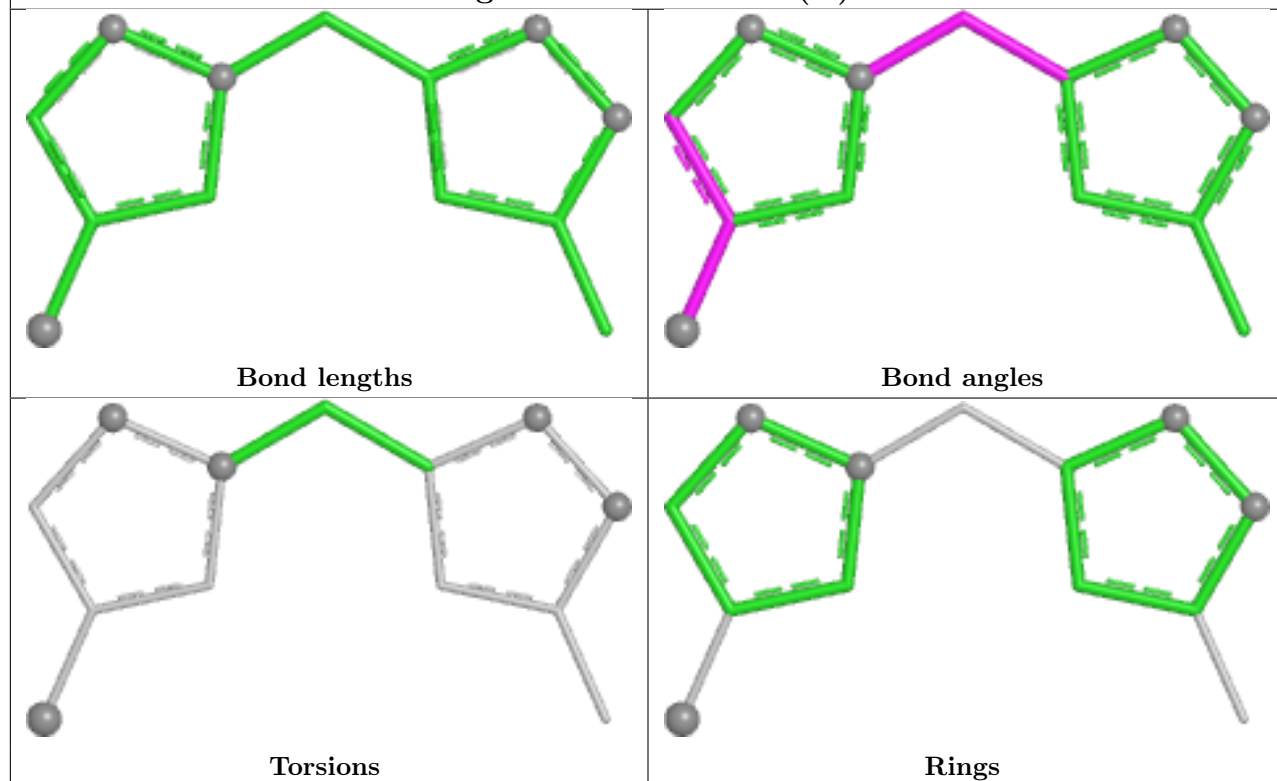
Ligand A1DN7 B 401 (A)
