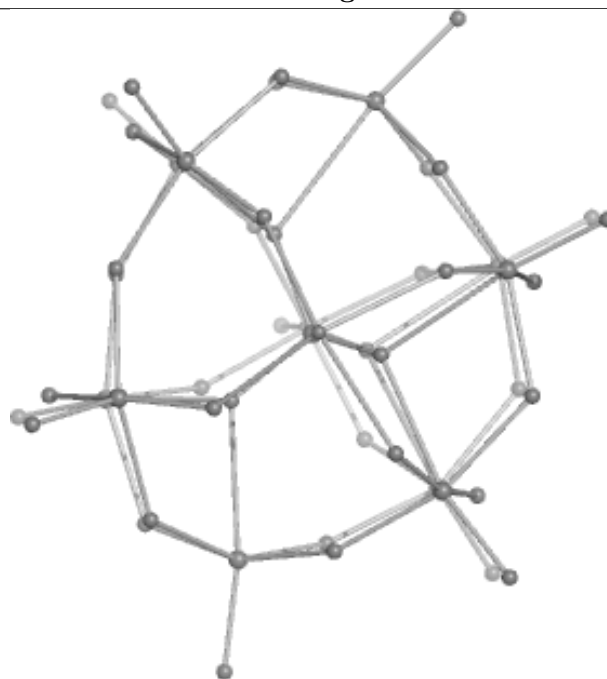
Rings
