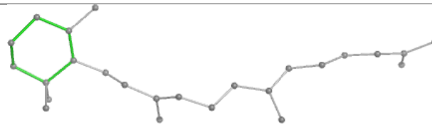
Rings
