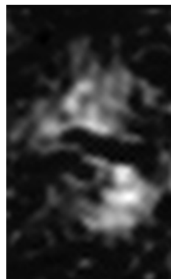
Z Index: 105
