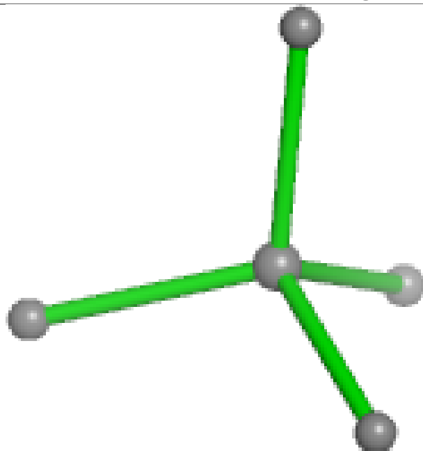
Bond lengths
